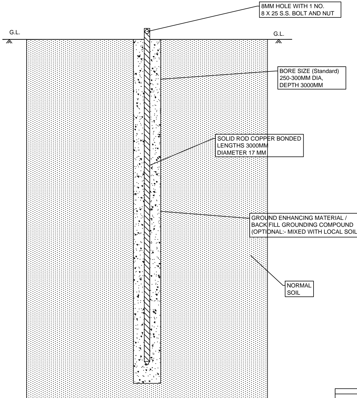
TOP VIEW OF THE ASSEMBLY (EARTH ROD AND 8X25 S.S. NUT BOLT)
