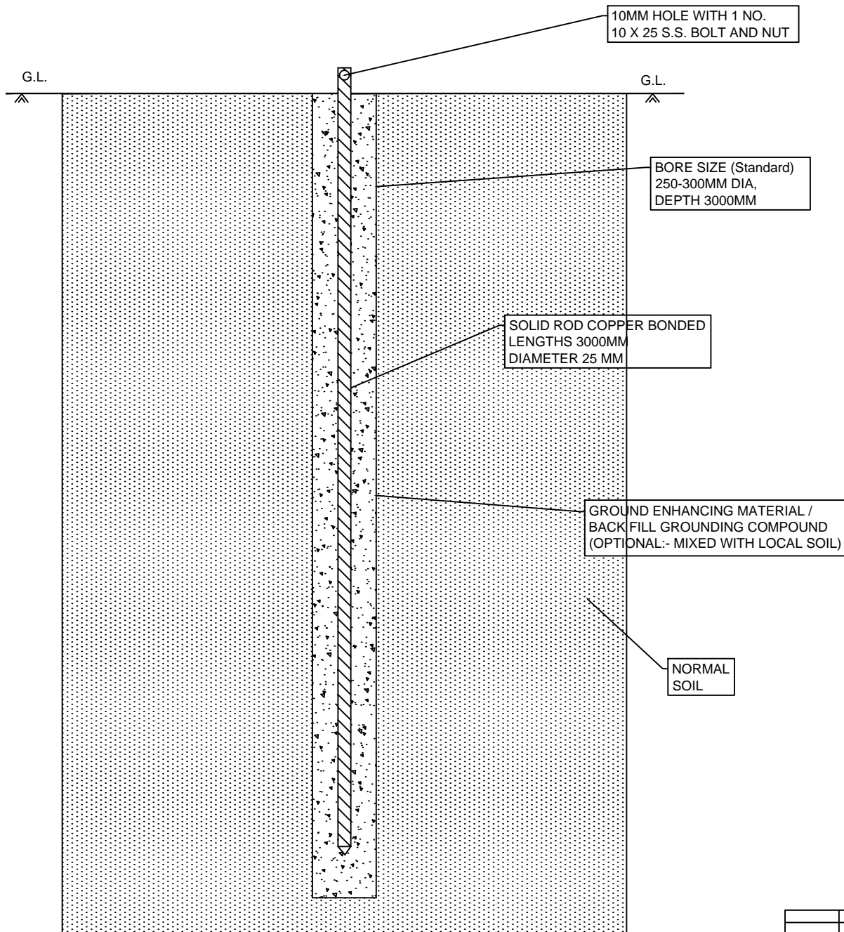
TOP VIEW OF THE ASSEMBLY (EARTH ROD AND 10X25 S.S. NUT BOLT)
