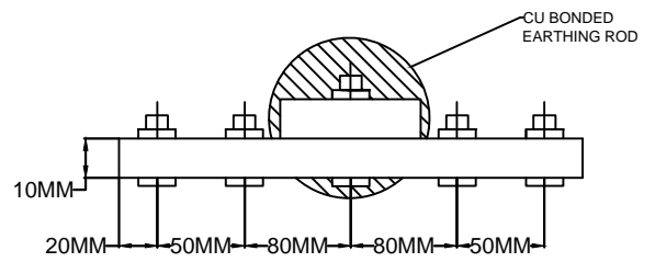
TOP VIEW OF THE ASSEMBLY (EARTH ROD AND TERMINATION ACCESSORIES) (OPTIONAL)
